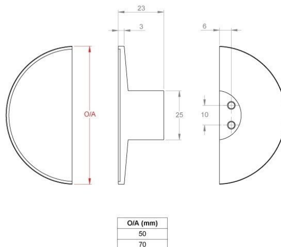
Dimensions drawing (DIM)
