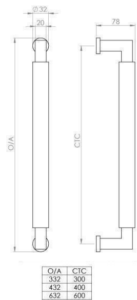
Dimensions drawing (DIM)
