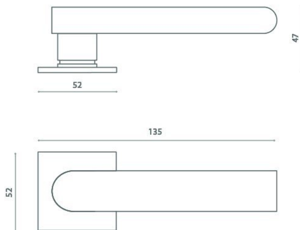
Dimensions drawing (DIM)
