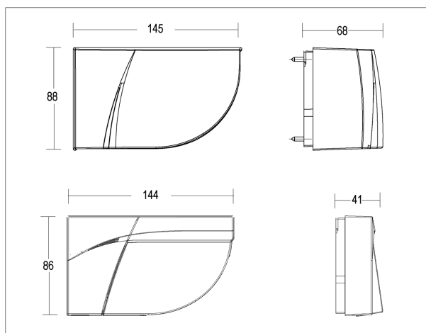
Dimensions drawing (DIM)
