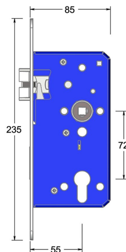
Dimensions drawing (DIM)
