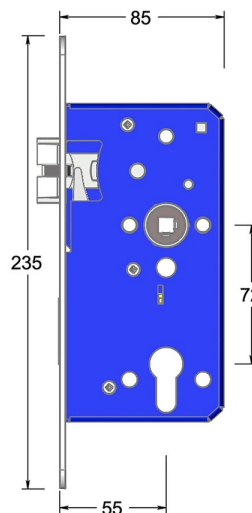
Dimensions drawing (DIM)
