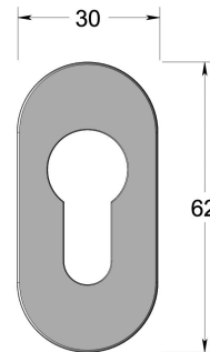
Dimensions drawing (DIM)
