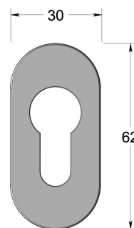
Dimensions drawing (DIM)
